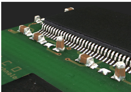
Reliable detection of defects such as tombstoning
